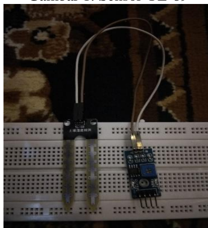
Gambar 1. Sensor YL-69
